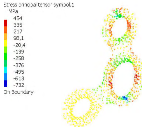
Figure 9. Compression and/or extension after force application.
