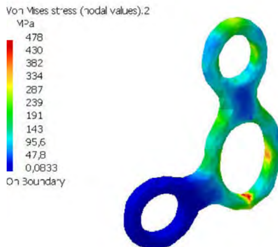
Figure 8. Von Mises stress distribution.
