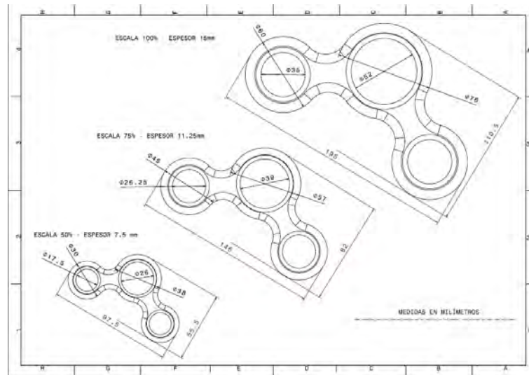
Figure 4. New descender layout in different scales.
