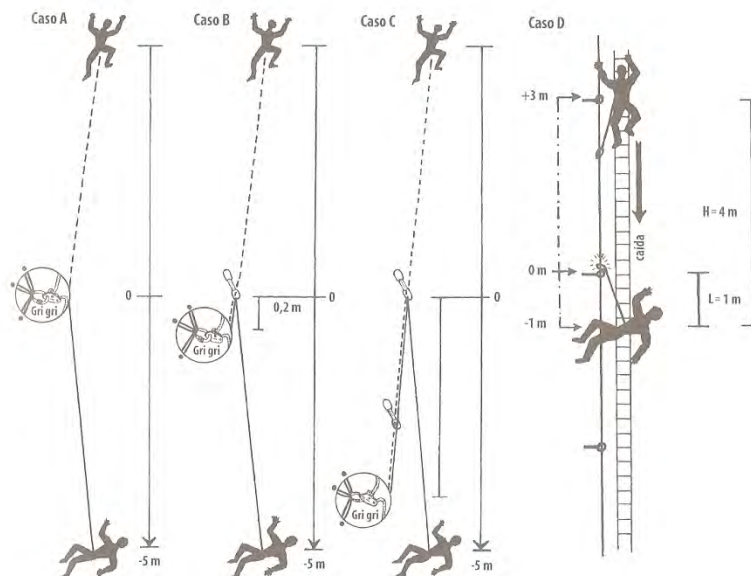
Figure 1. Impact force (see Bianchi et al., 2003, p. 17)
