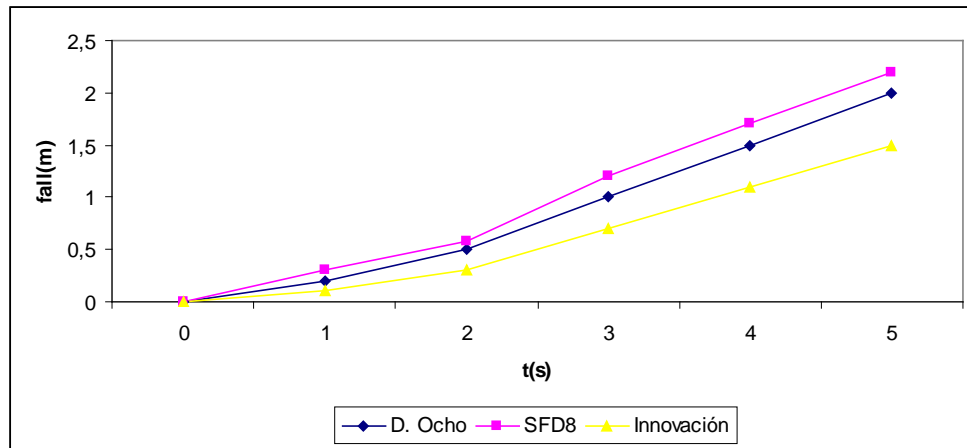
Figure 10. Difference of fall of a 80 kg weight in relation to the descender used.
