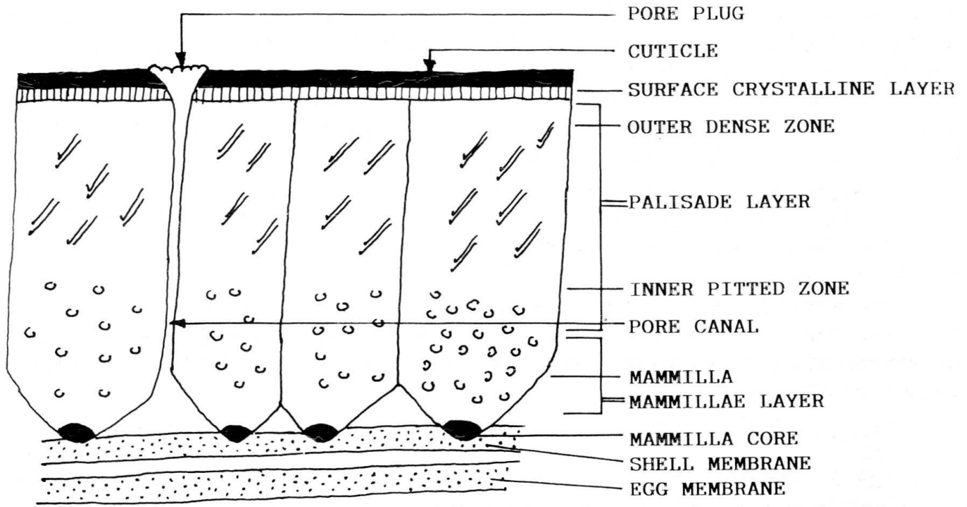
FIGURE 1 - Cross section of eggshell
