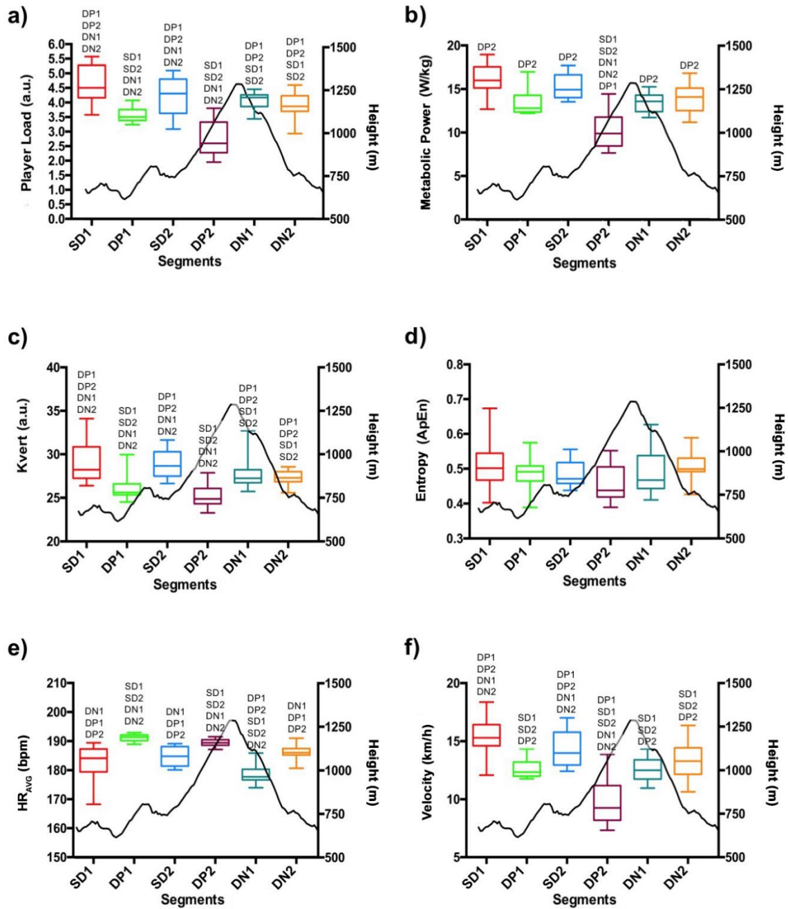
Figure 2. Box and whiskers plot and significant differences among segments depending of terrain slope in the load demands during an official mountain running race: (a) Player Load (PL), (b) Metabolic Power (MP), (c) Stiffness ( K_{VERT} ), (d) Approximate entropy (ApEn), (e) Heart rate ( HR_{AVG} ) and (f) Velocity ( V ).
